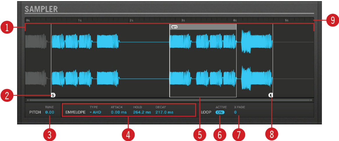
Sampler plug-in.
